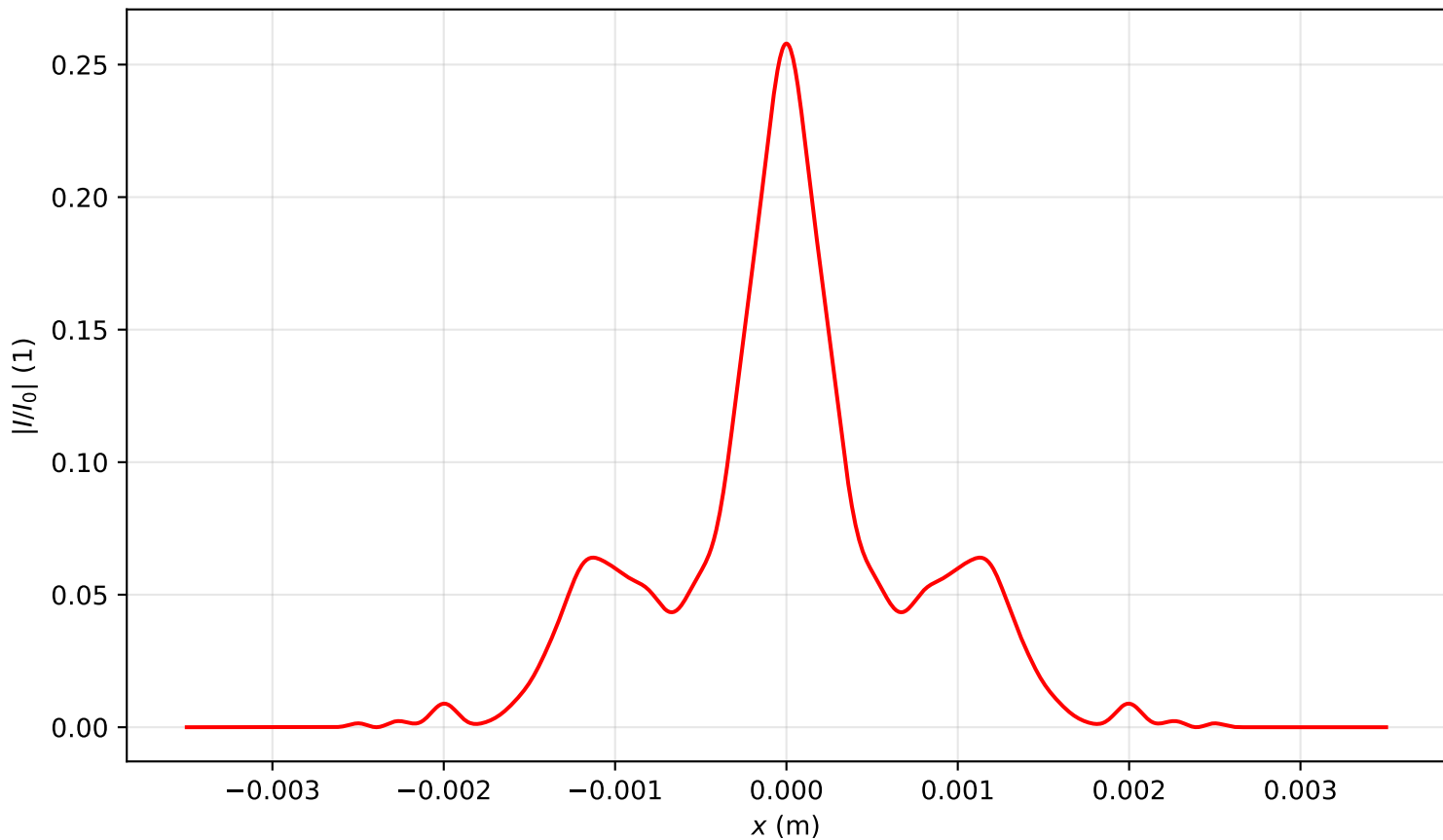
Intensity profile I(x, y = 0, z = 2.866)/I_0 , P_{in}=5.5P_{cr} , artificial time
